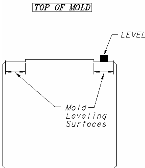
Fig.1 - PLAN VIEW
